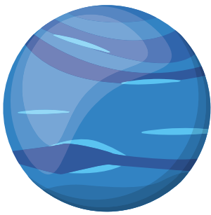
Neptune
