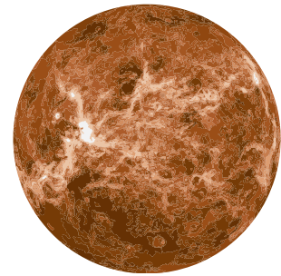
Mercury
