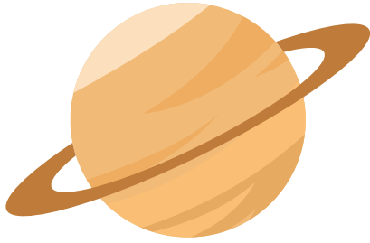
Saturn
